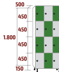
FCP-30/3 COD: 53529 97kg · 0,80m 3
