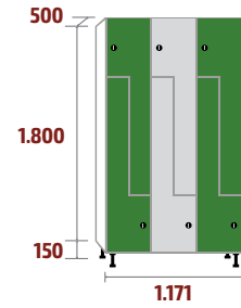
FLP-40/3 COD: 53630 117kg · 1,05m 3
