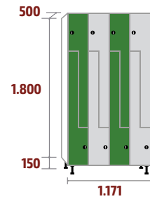
FLP-30/4 COD: 53629 132kg · 1,07m 3
