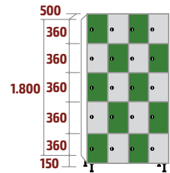
FPP-30/4 COD: 53617 138kg · 1,07m 3
